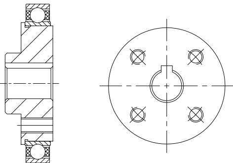
Keyway Type
