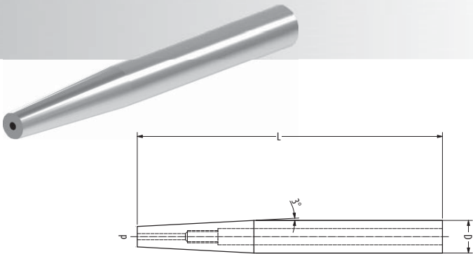
SHRINK FIT EXTENSIONS SLIM
