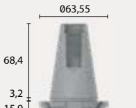
SK 40 DIN69871A/B Cod. 2AK
