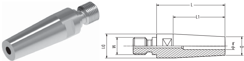
EXTENSIONS FROM MODULAR TO SHRINK FIT
